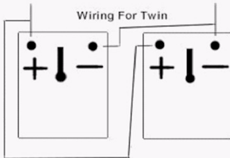
Twin Dry Fuel Cells In Parallel
