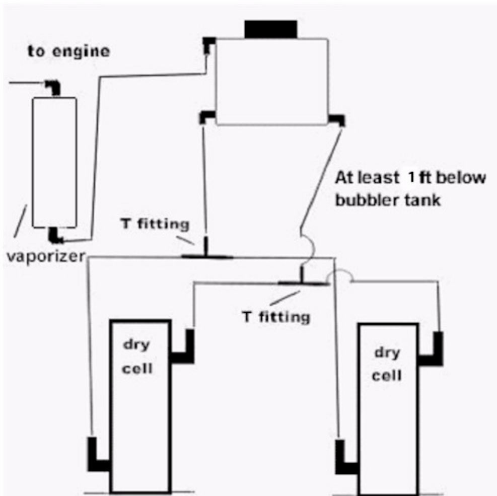
Twin Dry Fuel Cells In Parallel
